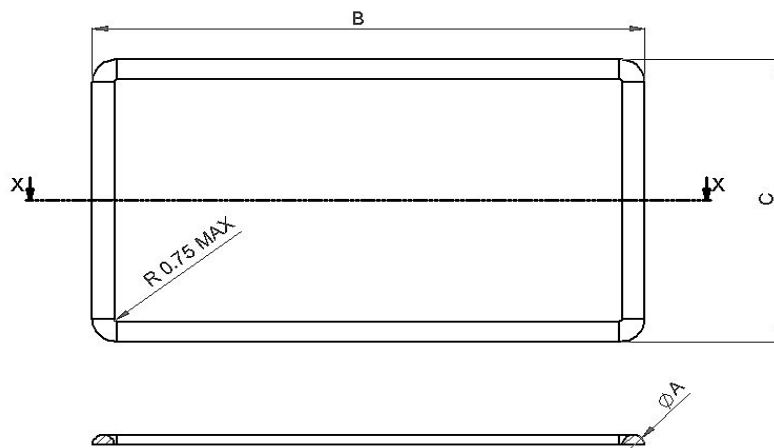
SECTION X-X
